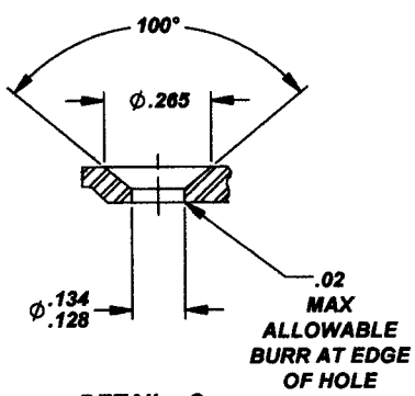
DETAIL - C COUNTERSINK MOUNTING HOLE
