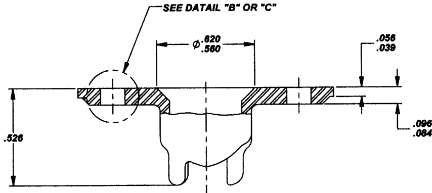
DETAIL - A
